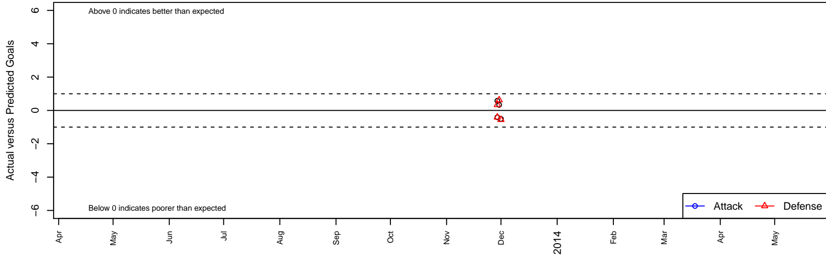
Futeca Camp Elite B96 Dots are actual minus expected GF (blue circles) and GA (red triangles). Blue line is smoothed change in attack strength. Red is smoothed change in defense strength.
